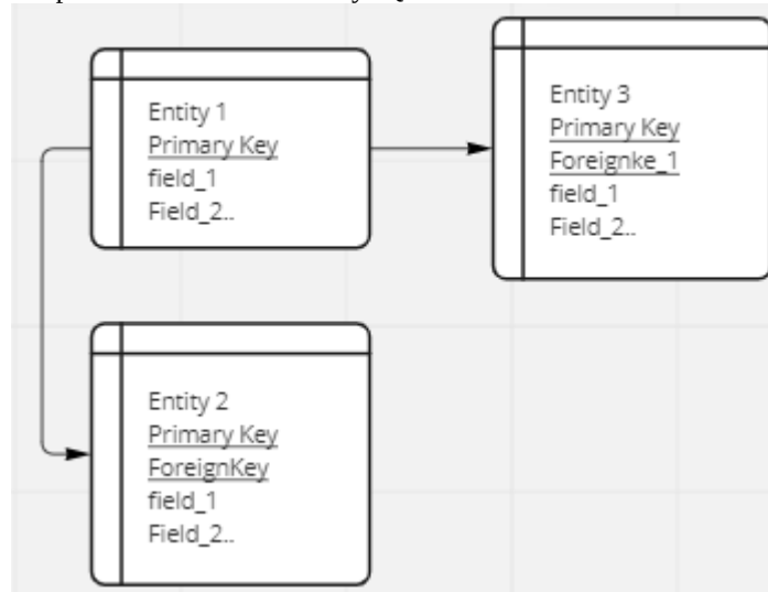
Fig 3. Relational design in RDBMS
