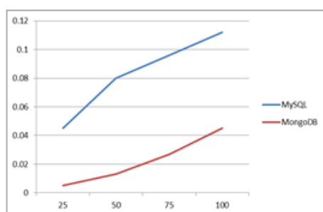
Fig. 9. Comparison of insert times
