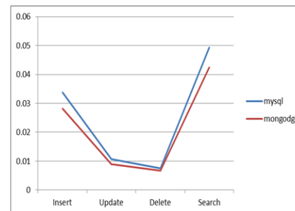
Fig. 13. Performance comparison of MySQL and MongoDB
